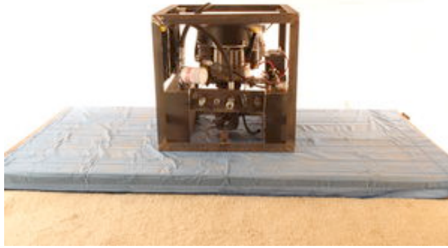
Figure 2. The OSE “power cube” is a modular hydraulic power source used to power many of the machines in the GVCS. Like all OSE machines, it is designed to be inexpensive to build, simple to repair, and easily adapted to a variety of purposes. Image courtesy of Open Source Ecology (CC-BY-SA).
